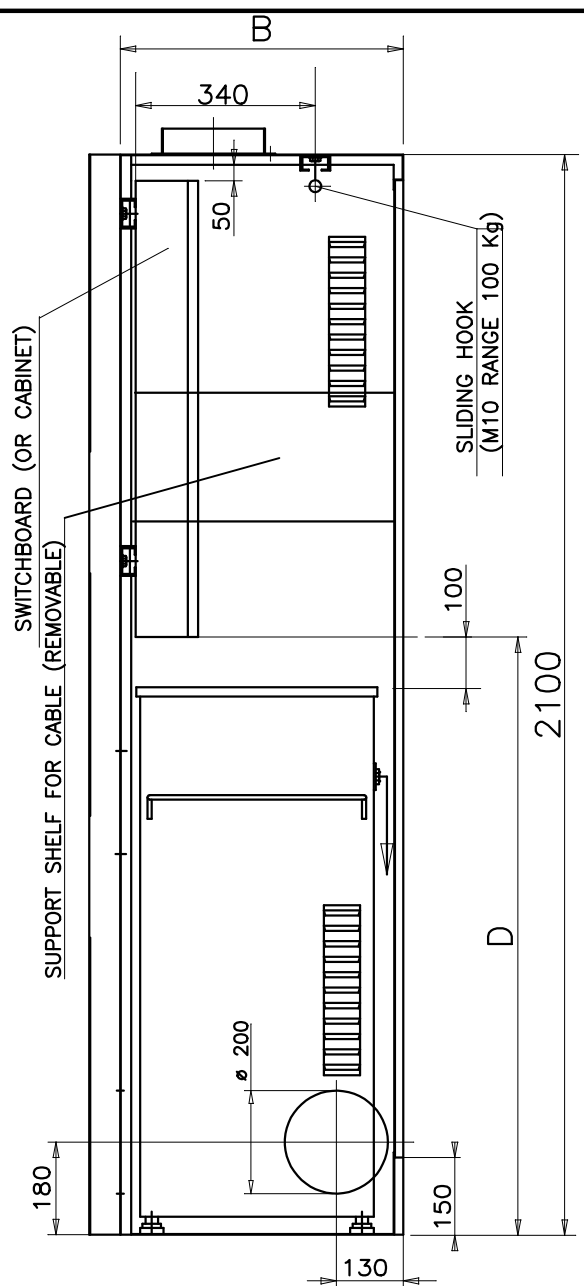
SECTION: X-X
